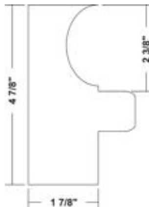
CAR-BN-RC-FG-APC
