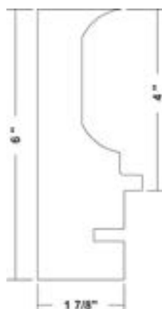
CAR-ICC-FGWT
